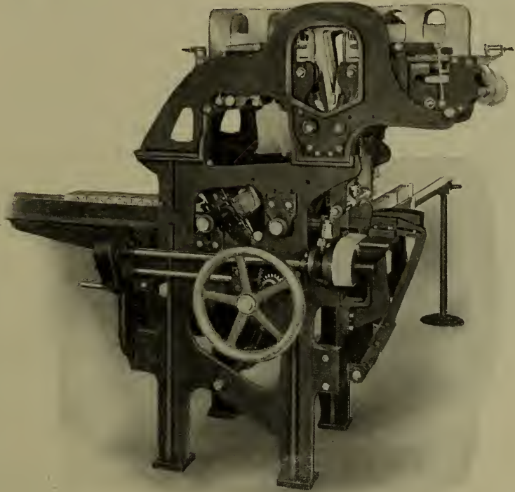
Style D Sheet Feed Wrapping Machine.
